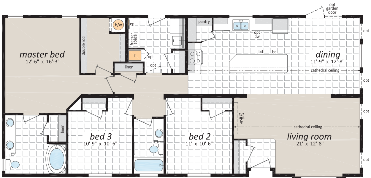
Kent - ST-7601 27' x 60' • 1,620 sq. ft. 3 Beds | 2 Baths
